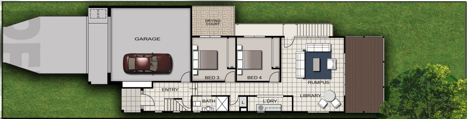
LOWER FLOOR PLAN
