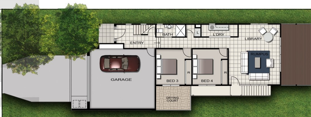
LOWER FLOOR PLAN
